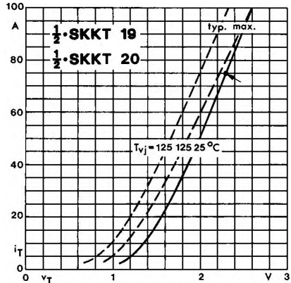
Fig. 8 On-state characteristics
