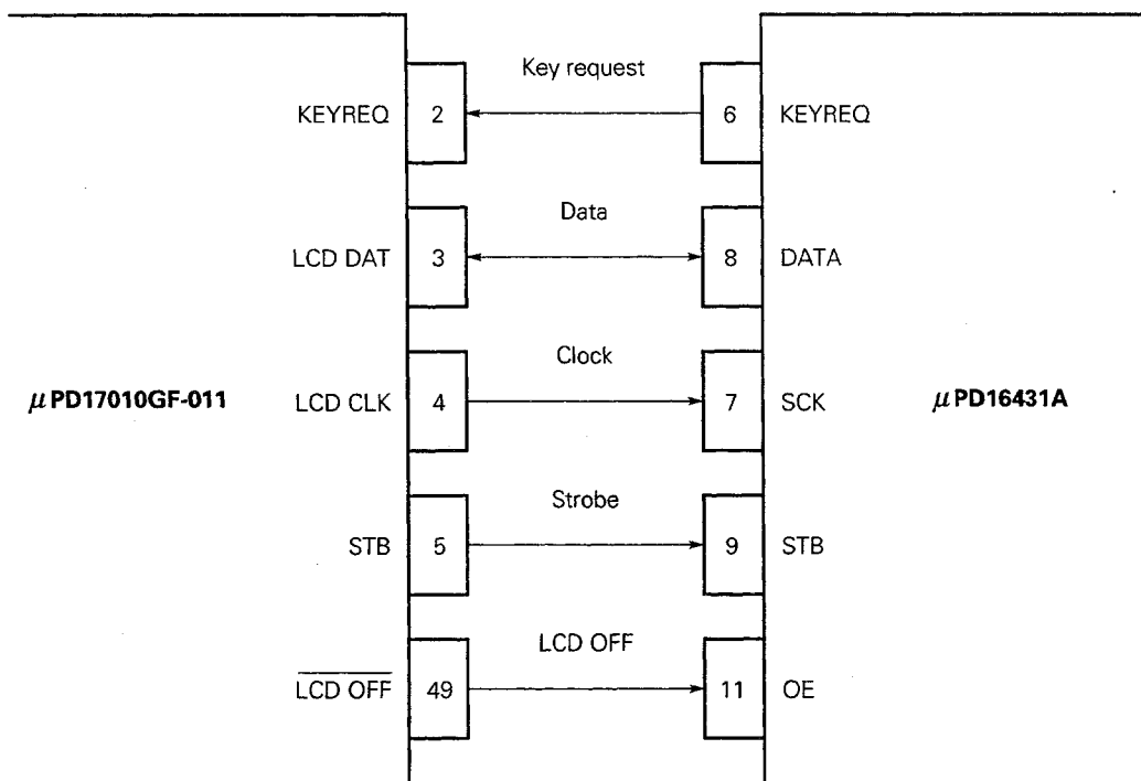
Fig. 4-1 \mu PD16431A Pin Configuration
