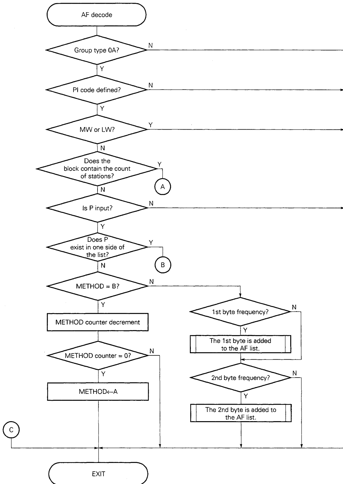
Fig. 5-3 Flow of AF List Input (1/3)
