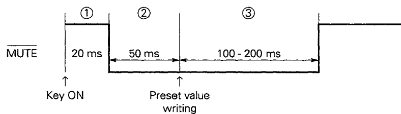
Fig. 6-3 Timing Chart in Preset Memory Write
