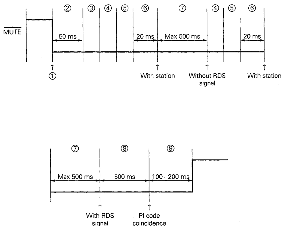
Fig. 6-12 Timing Chart of Switchover to EON Station (if the preset memory contains the same PI code as the EON station)
