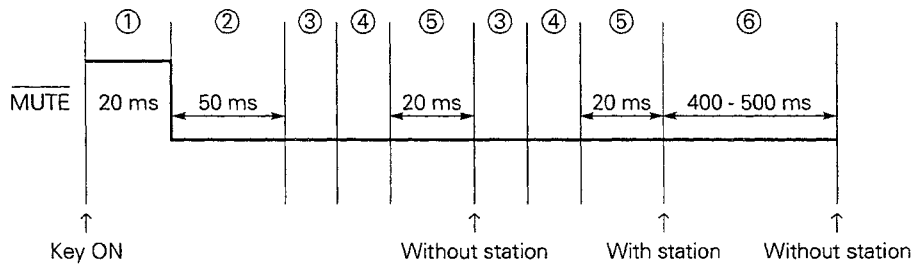
Fig. 6-5 Timing Chart in Seek Up/Down (RDS Mode)
