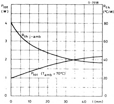
Figure 16 : Maximum Dissippable Power and Junction to Ambient Thermal Resistance vs. Side " \alpha ".
