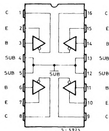
ULN2074B ULN2076B
