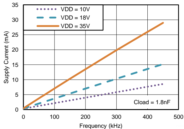
Figure 8. Operating Supply Current vs. Frequency
