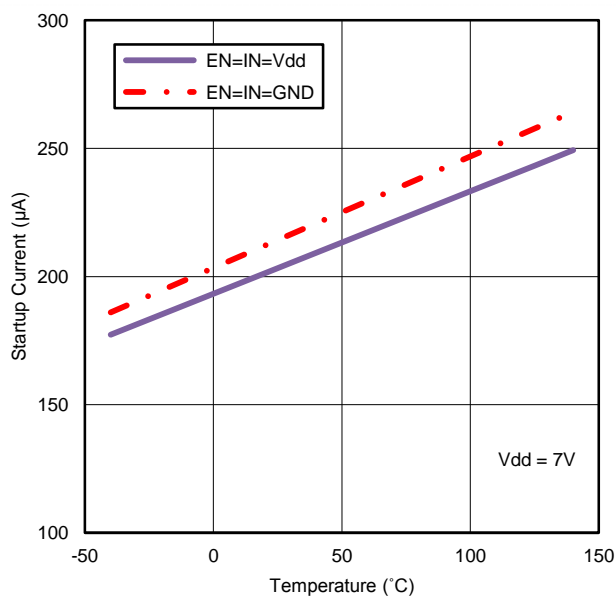
Figure 9. Start-Up Current vs. Temperature
