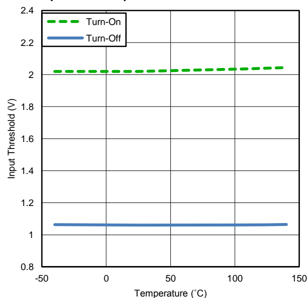
Figure 12. Input Threshold vs. Temperature
