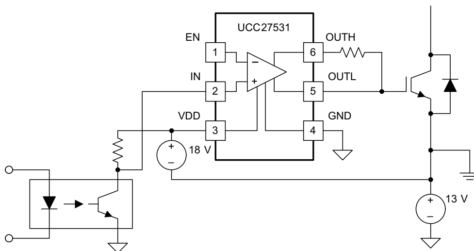
Figure 3. Driving IGBT With 13-V Negative Turn-Off Bias
