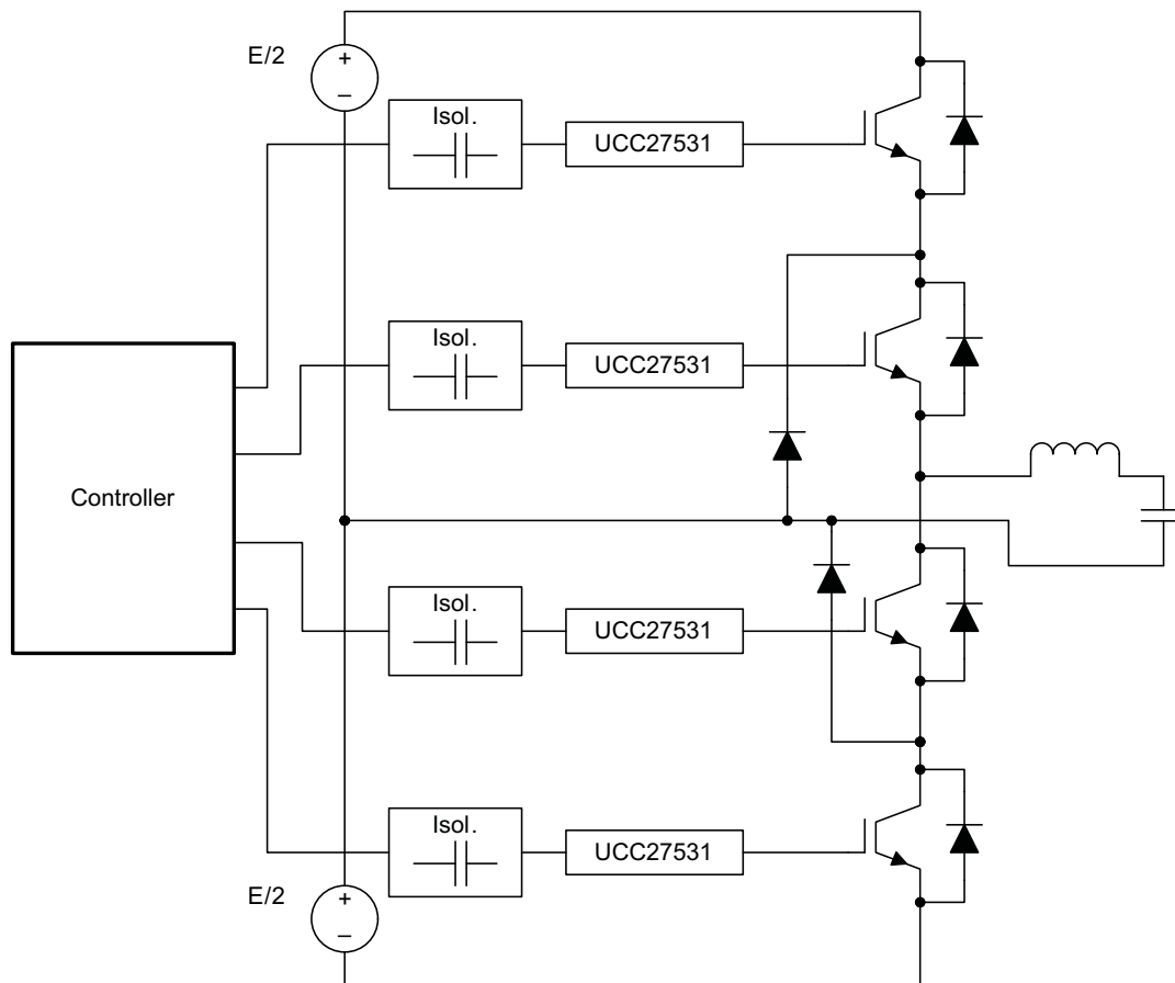
Figure 4. Using UCC27531 Drivers in an Inverter
