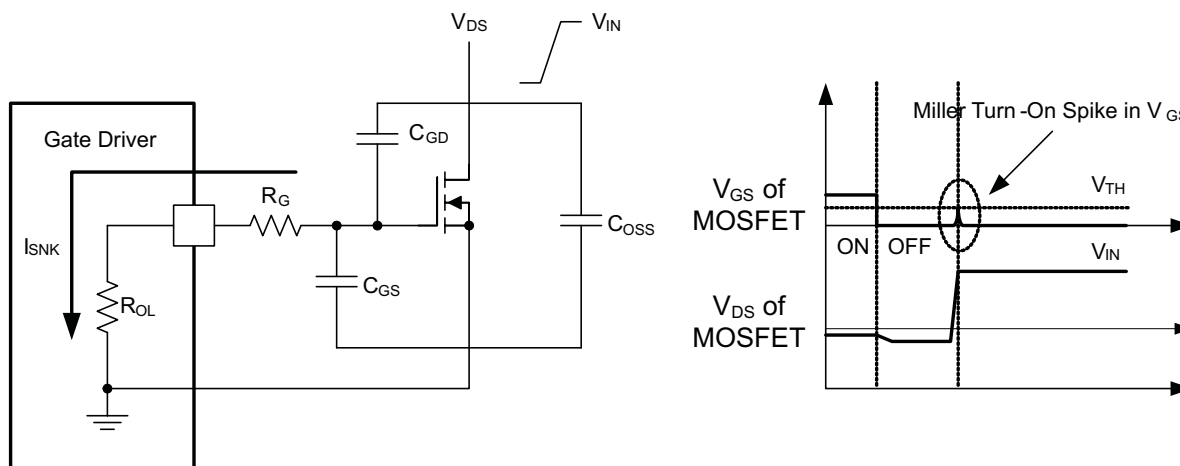
Figure 25. Low Pull-Down Impedance in UCC27531 (output stage mitigates Miller turn-on effect)
