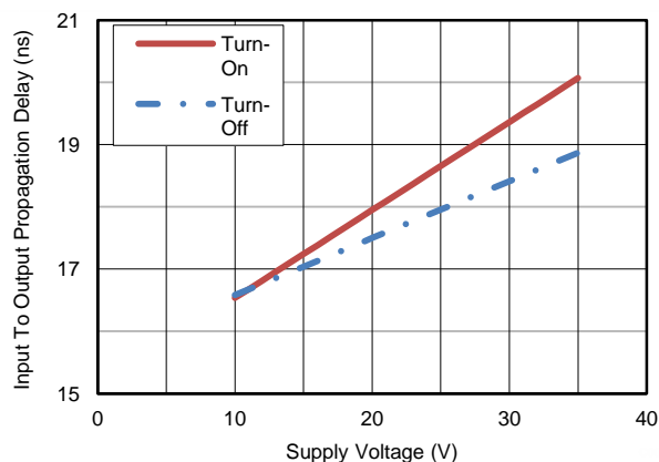
Figure 7. Propagation Delay vs. Supply Voltage
