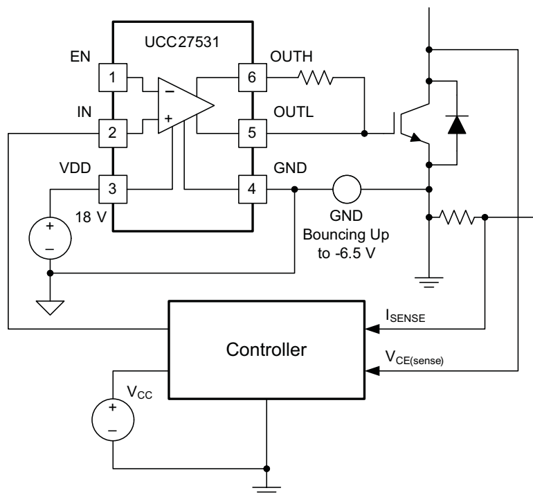
Figure 2. Driving IGBT Without Negative Bias
