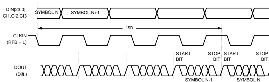
Figure 9. Serializer Latency Delay
