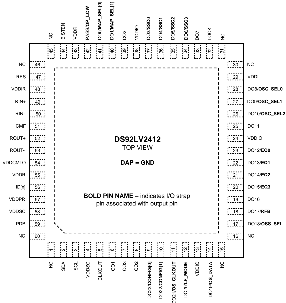
Figure 2. Deserializer - DS92LV2412 — Top View
