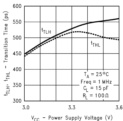
Figure 23. Transition Time vs Power Supply Voltage
