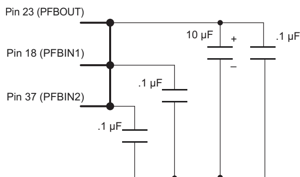
Figure 7-3. Power Feedback Connection
