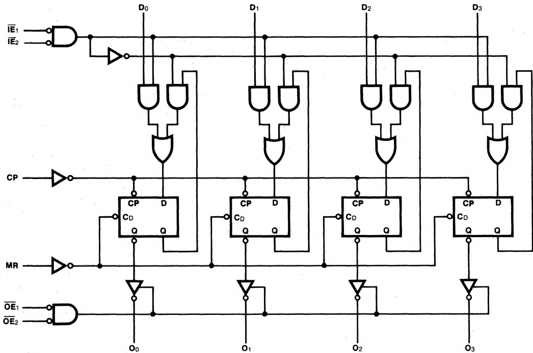
LOGIC DIAGRAM
