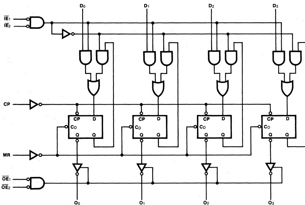
LOGIC DIAGRAM
